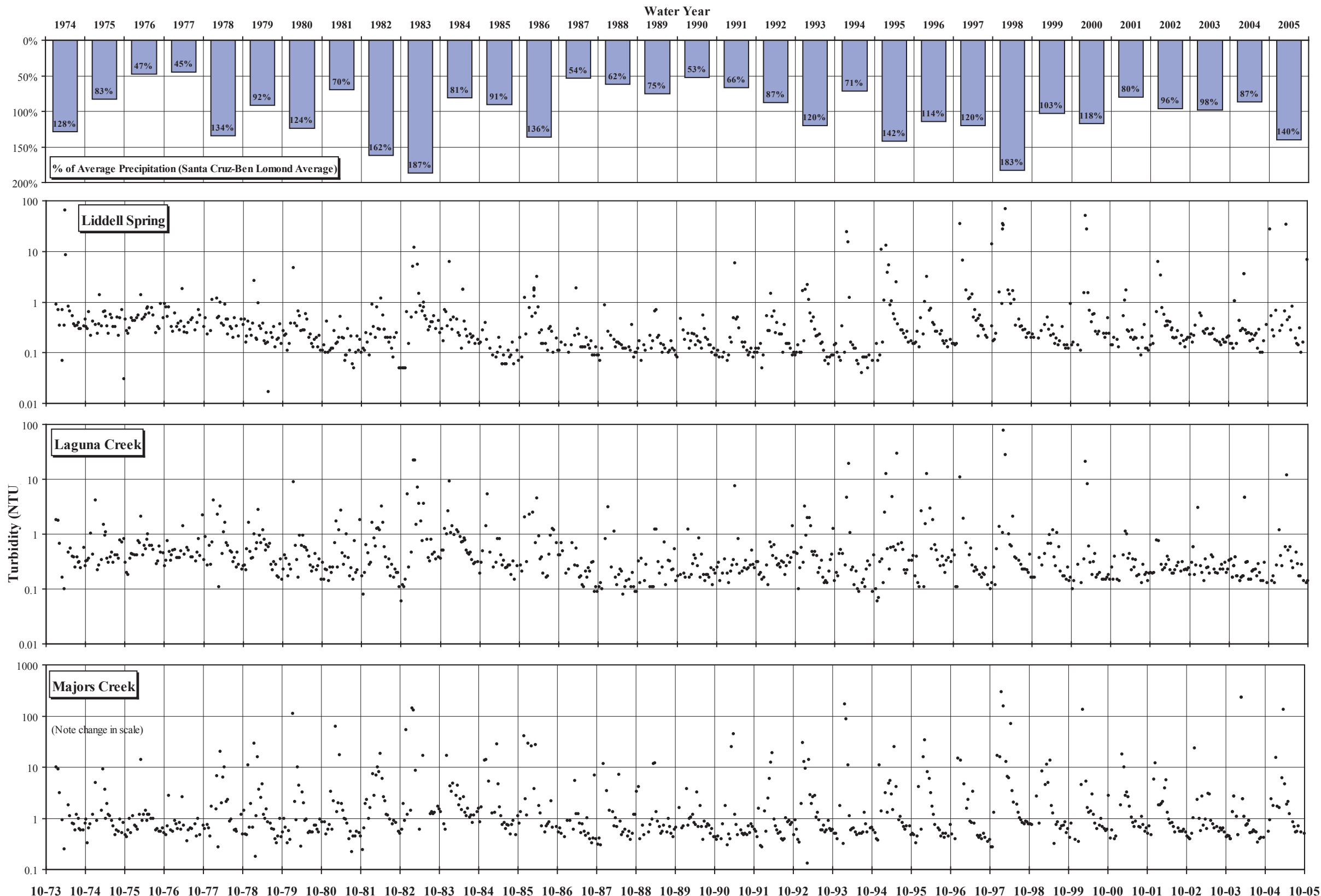
Turbidity of North Coast Diversions, WYs 1974-2005
